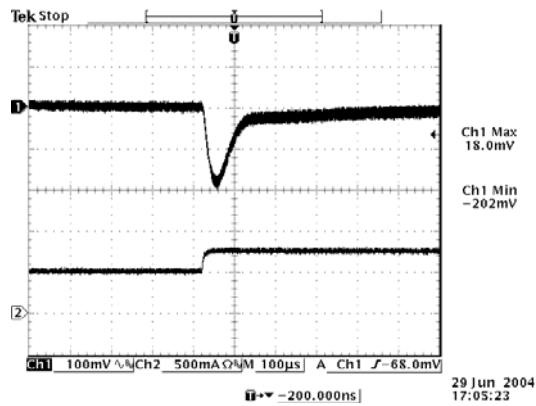
50% to 75% load transient at 5 Vdc output
