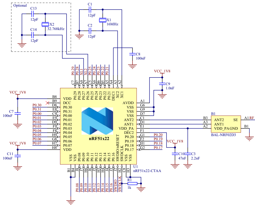
Figure 43 CTAA WLCSP with low voltage mode setup
