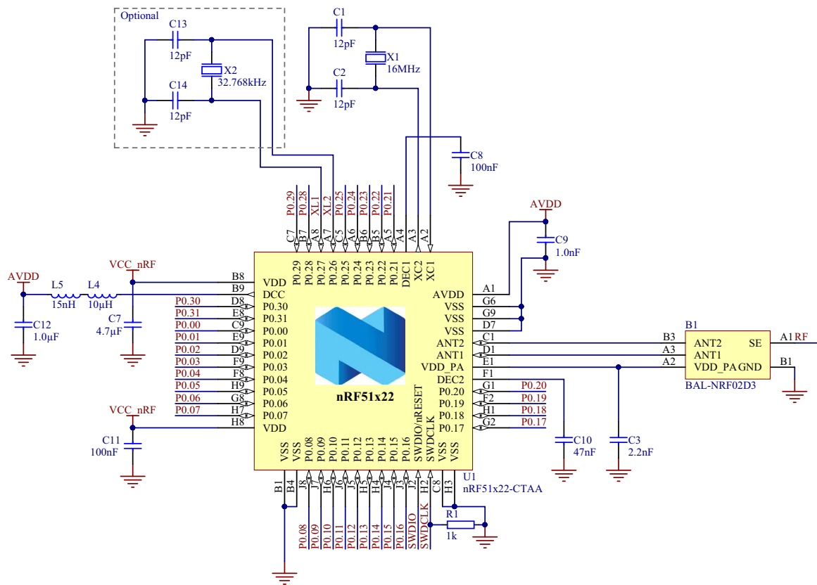
Figure 44 CTA/WLCSP with DC/DC converter setup
