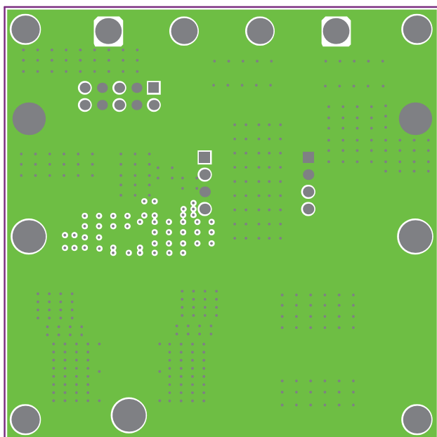
Figure 3: Mid Layer 2
