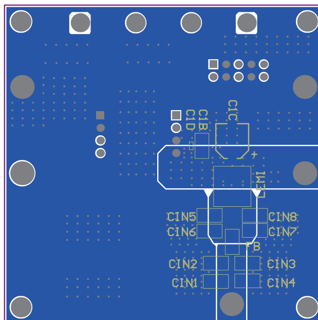
Figure 4: Bottom Layer
