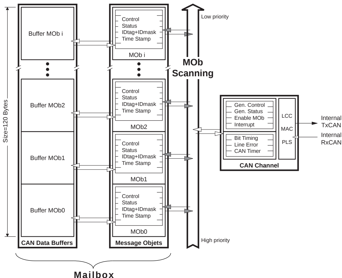
Figure 19-5. CAN Controller Structure
