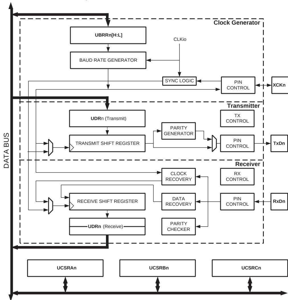
Figure 17-1. USARTn Block Diagram (1)
