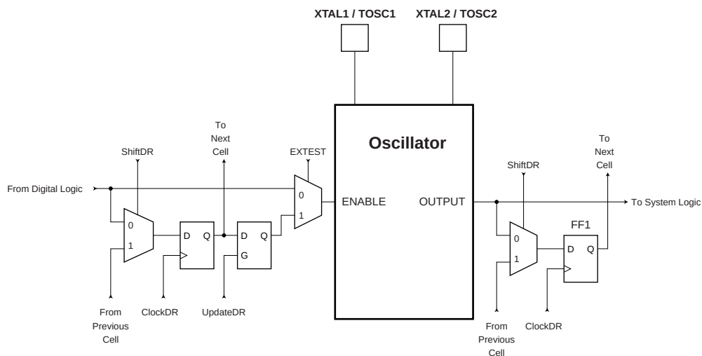
Figure 23-7. Boundary-scan Cells for Oscillators and Clock Options
