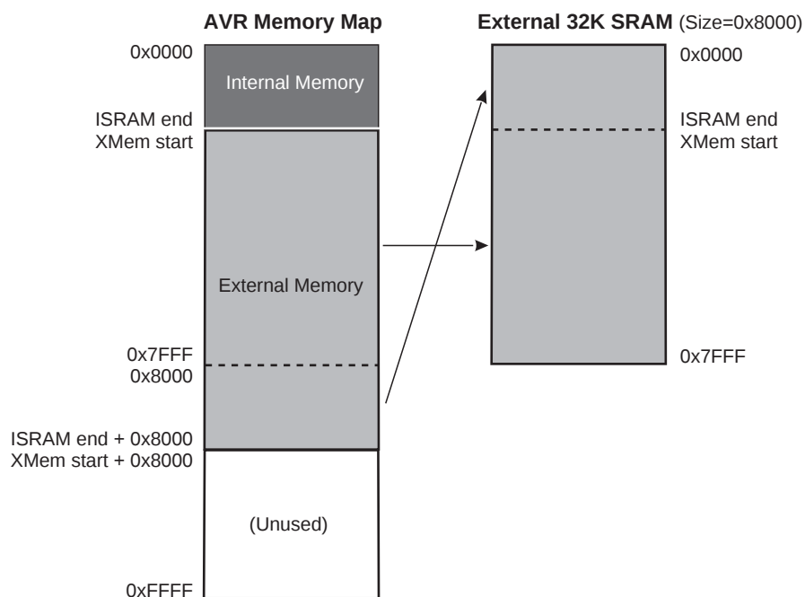
Figure 4-10. Address Map with 32 KB External Memory
