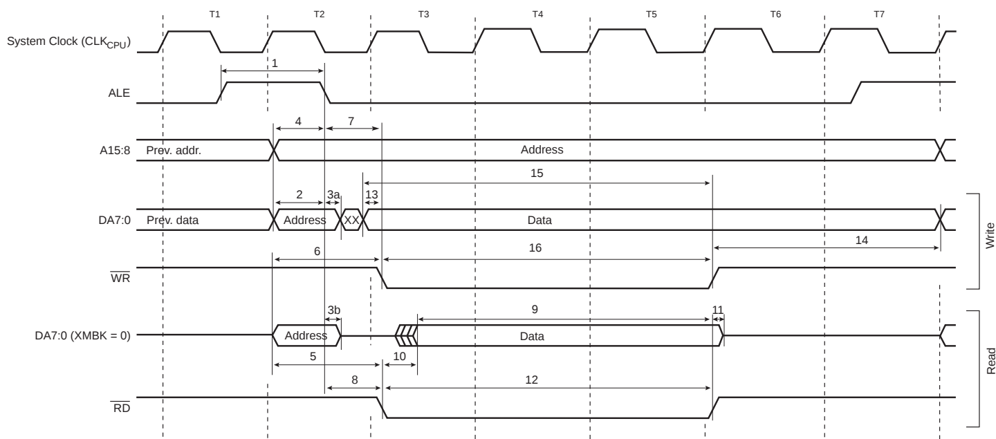
Figure 26-9. External Memory Timing (SRWn1 = 1, SRWn0 = 1) (1)
