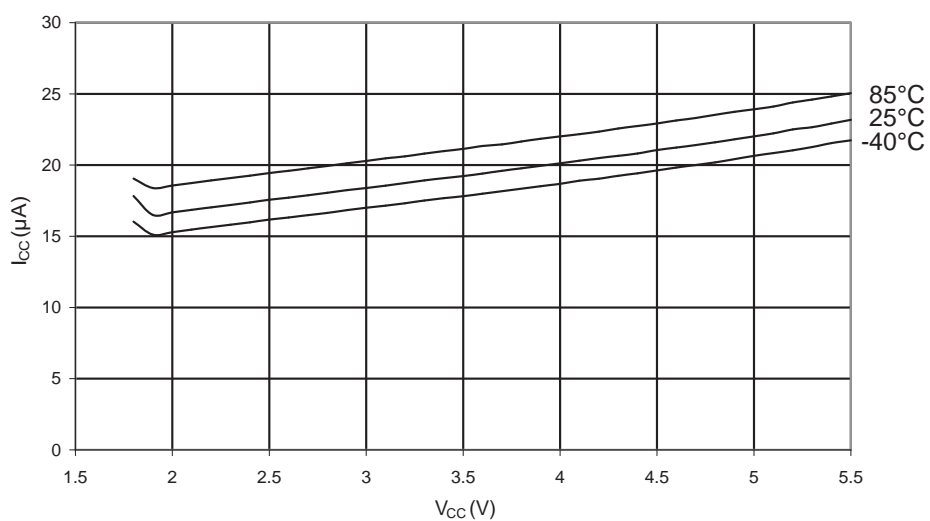
Figure 27-89. Brownout Detector Current vs. V_{CC}
