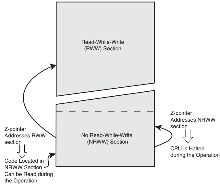
Figure 24-1. Read-While-Write vs. No Read-While-Write
