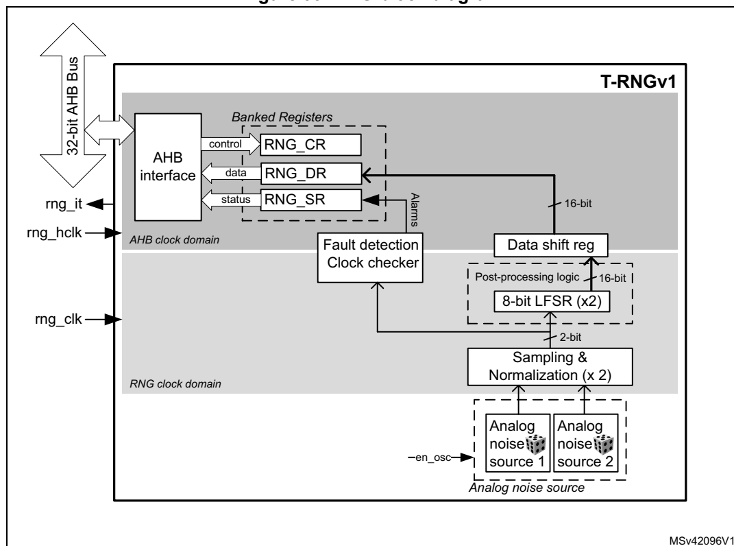
Figure 99. RNG block diagram
