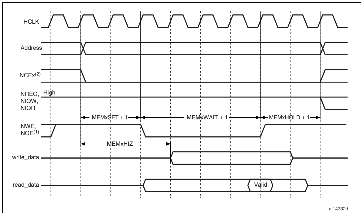
Figure 205. NAND/PC Card controller timing for common memory access
