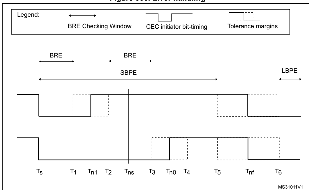
Figure 333. Error handling
