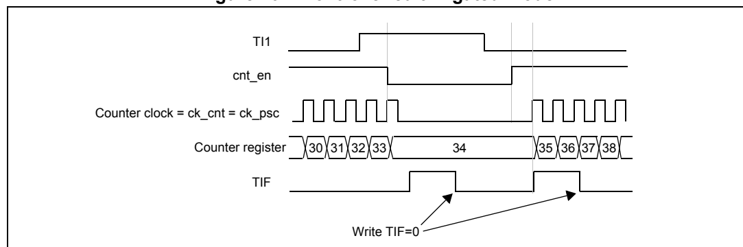
Figure 104. Control circuit in gated mode
