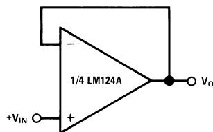
Figure 11. Voltage Follower
