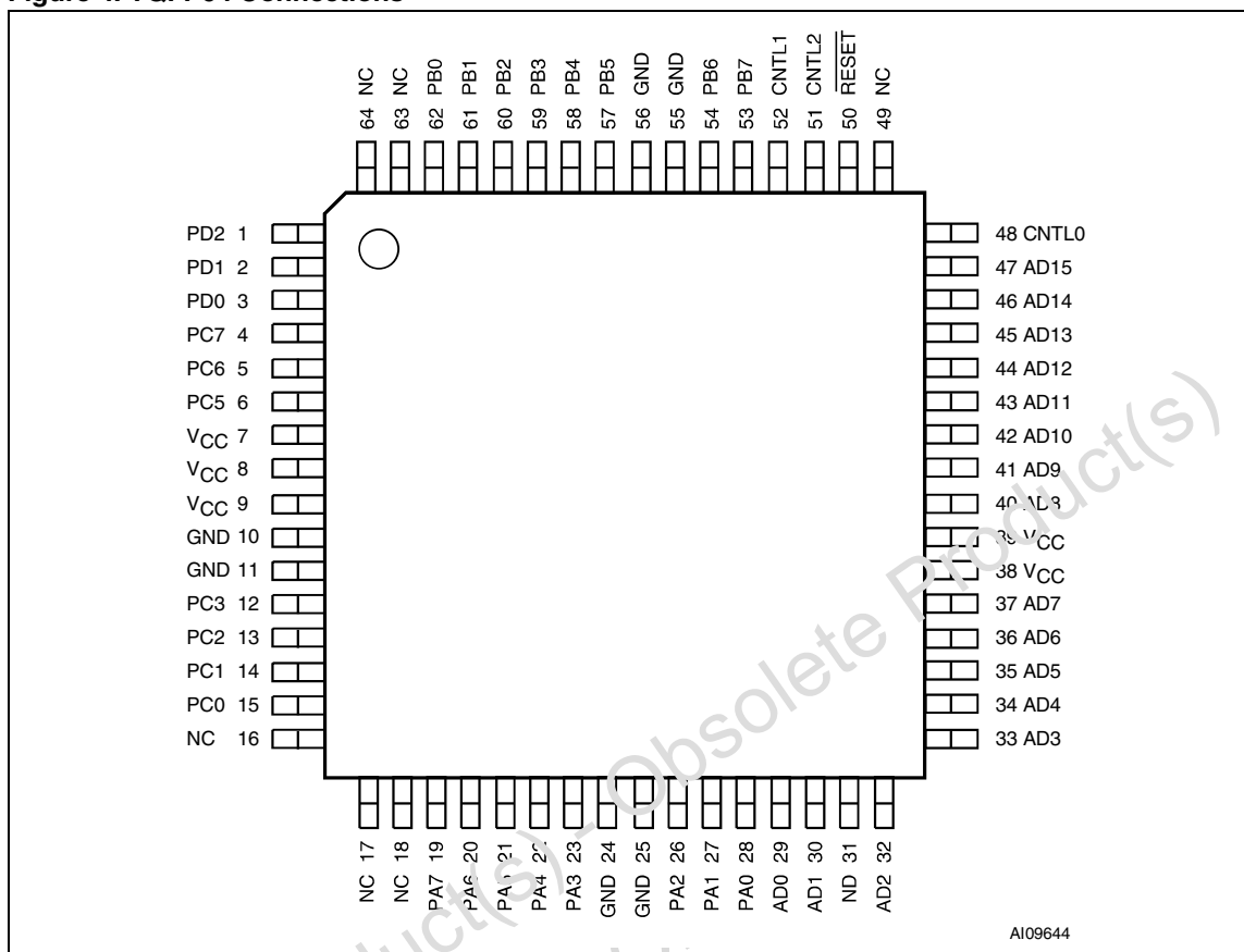
Figure 4. TQFP64 Connections
