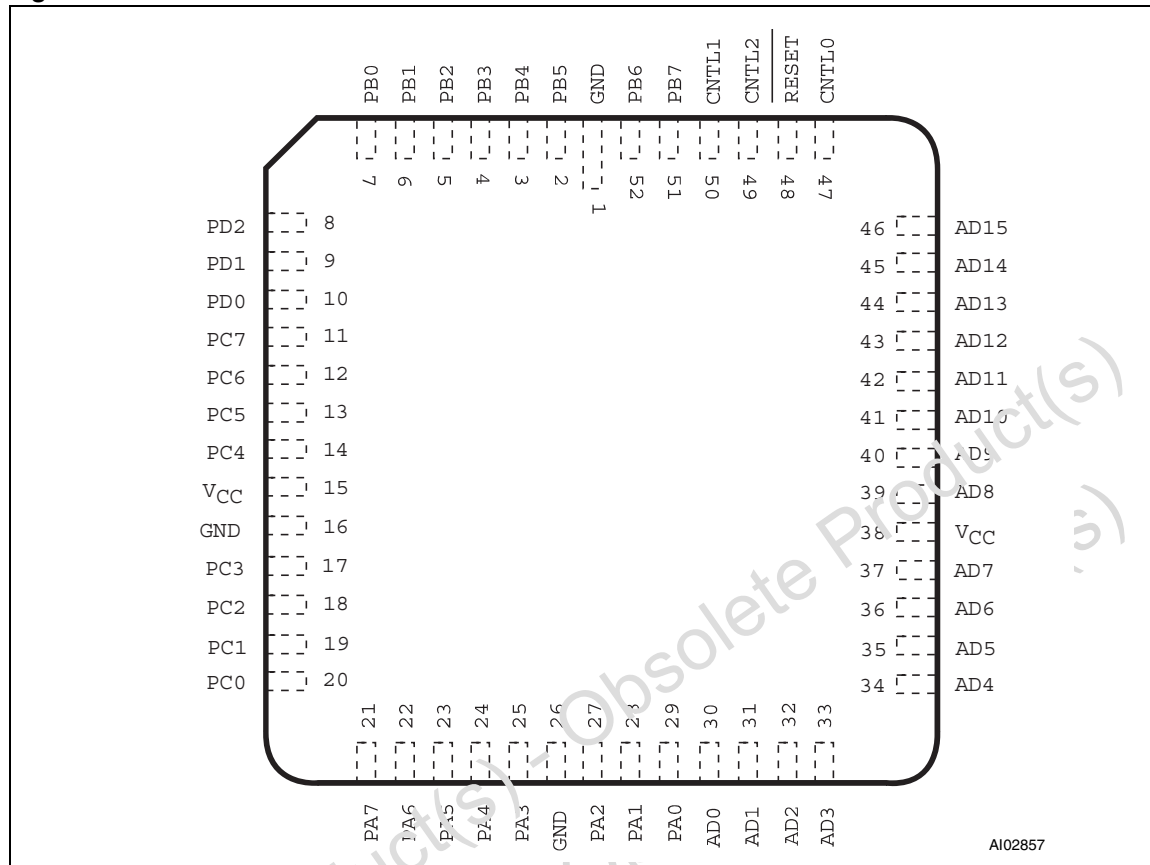
Figure 3. PLCC52 Connections
