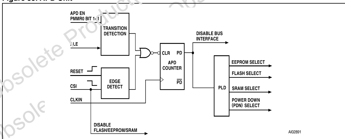
Figure 33. APD Unit
