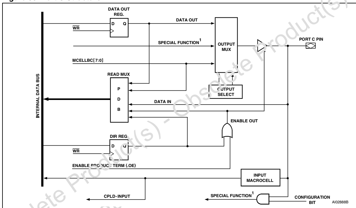
Figure 30. Port C Structure
