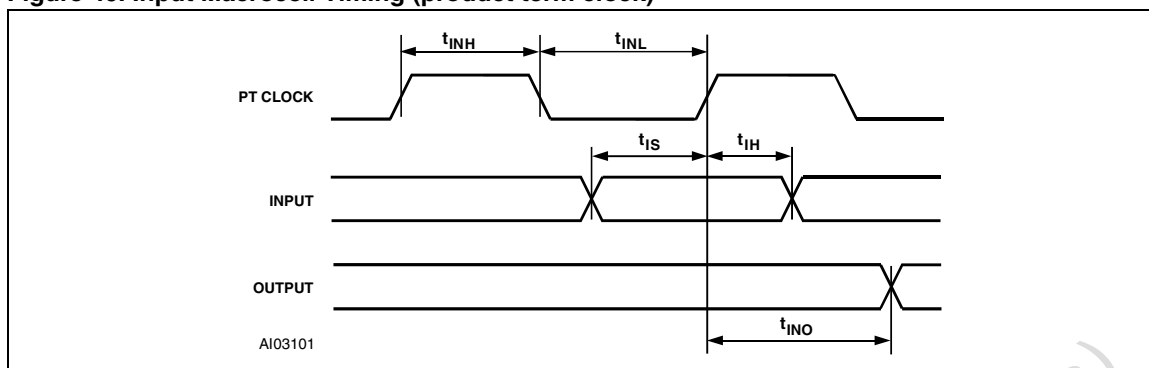
Figure 46. Input Macrocell Timing (product term clock)
