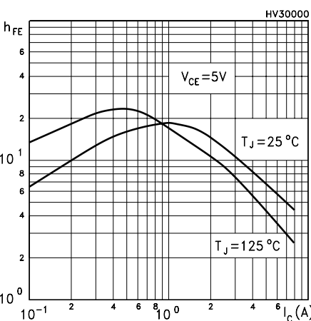
Figure 6. DC current gain
