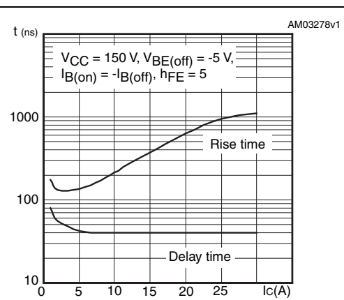
Figure 7. Resistive load switching times (on)
