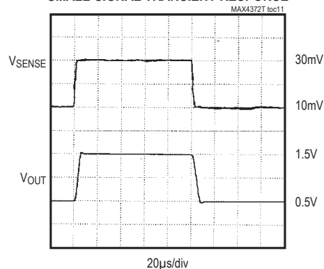
MAX4372F SMALL-SIGNAL TRANSIENT RESPONSE
