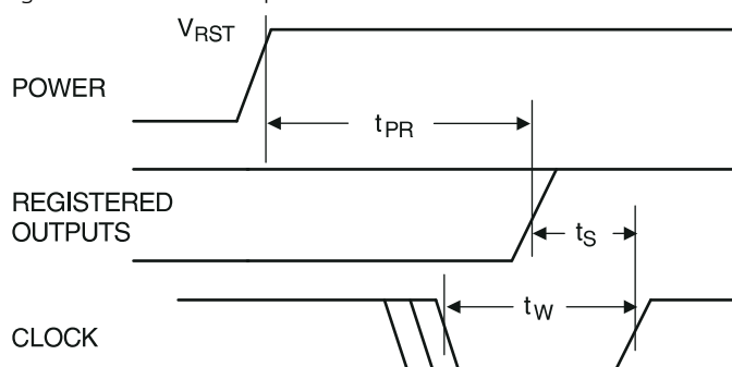
Figure 8. Power-up reset
