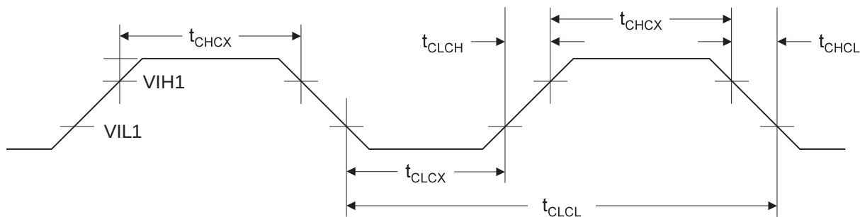
Figure 69. External Clock
