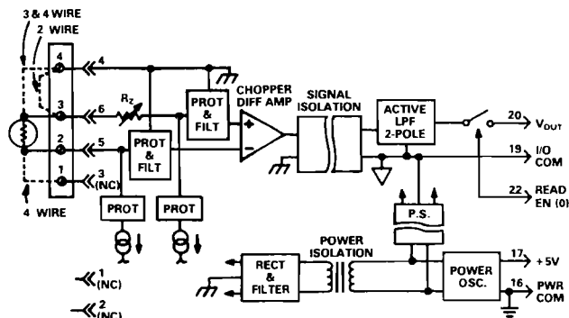
Figure 2.4. 5B34 Functional Block Diagram
