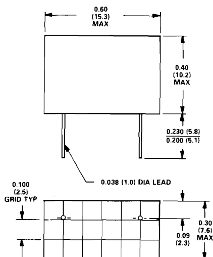
Figure 4.6. AC1362 Outline
