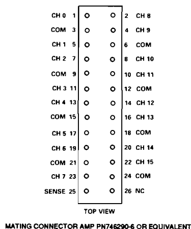
Figure 3.3. 5B01 System Connector Pinout
