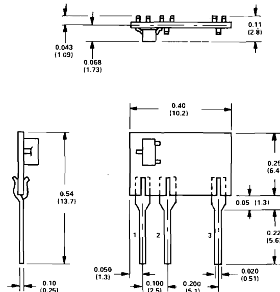
Figure 4.4. AC1361 Outline
