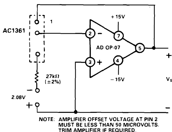
Figure 4.5. AC1361 Test Circuit
