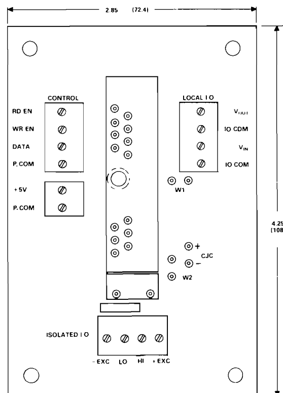
Figure 4.7. AC1360.
