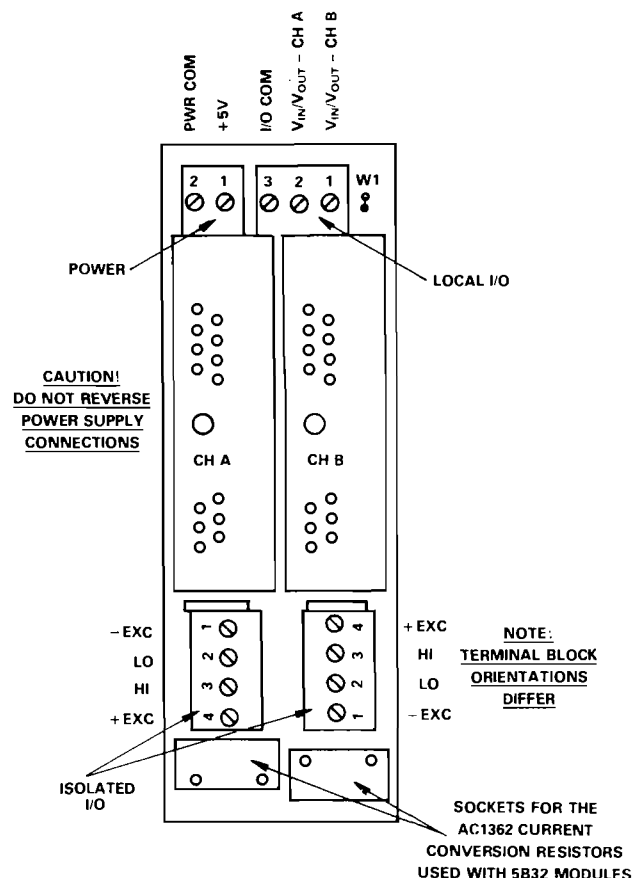
Figure 3.9. 5B04 Wiring
