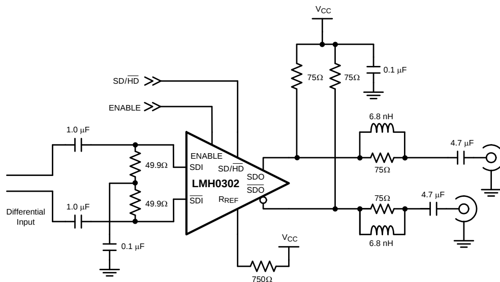
Figure 3. Application Circuit
