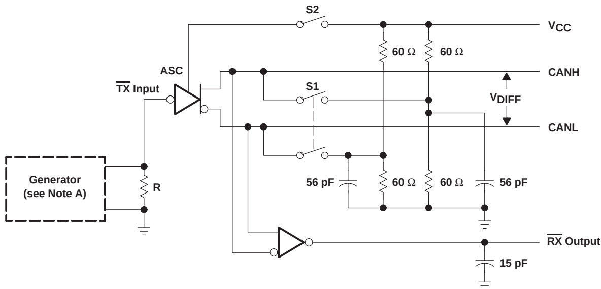
Figure 2. Test Circuit
