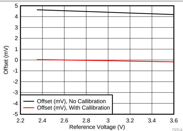
Figure 15. Offset vs Reference Voltage (AVDD)
