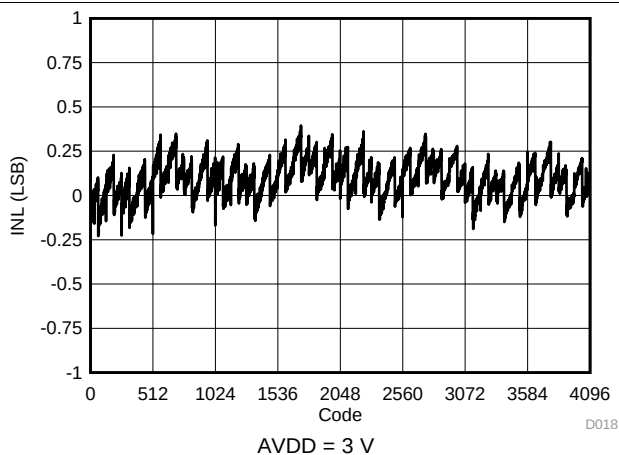
Figure 19. Typical INL
