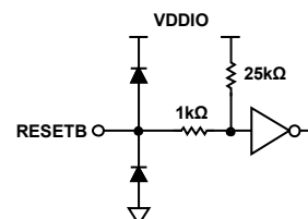
Figure 63. Equivalent RESETB Input Circuit
