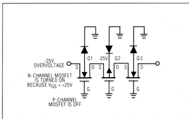
Figure 8. -25\text{V} Overvoltage with Multiplexer Power OFF
