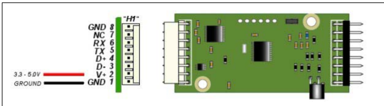
FIGURE 2-2: POWER
