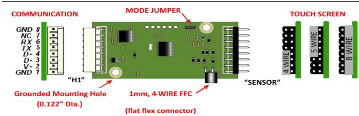
FIGURE 2-1: CONNECTIONS – OVERVIEW
