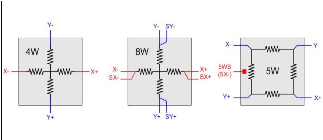
FIGURE 2-5: SENSOR CONNECTIONS
