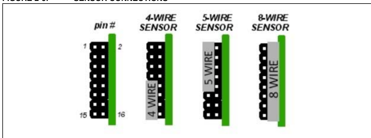
FIGURE 2-6: SENSOR CONNECTIONS
