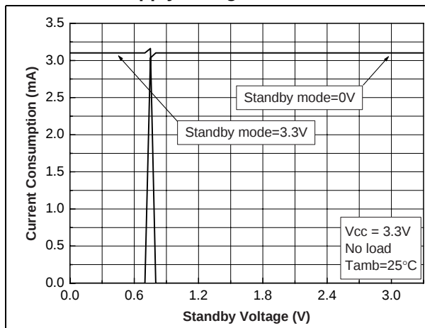
Figure 5. Current consumption vs. power supply voltage
