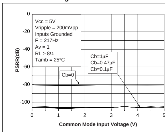
Figure 31. PSRR vs. common mode input voltage
