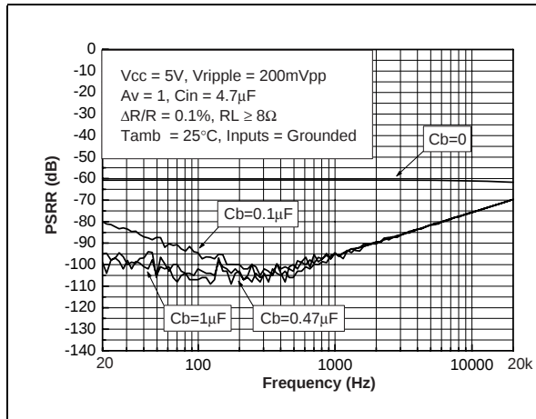
Figure 70. PSRR vs. frequency (worst case conditions)
