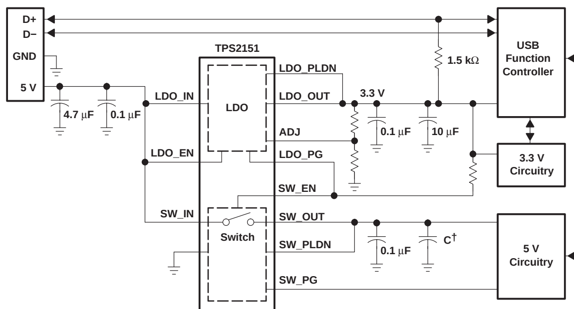
Figure 27. Bus-Powered USB Peripheral Application
