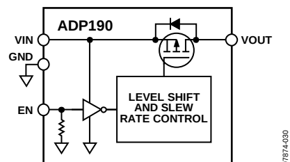
Figure 17. ADP190 Functional Block Diagram
