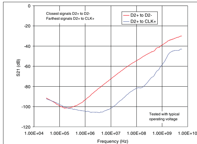
Figure 7. Channel-to-Channel Crosstalk
