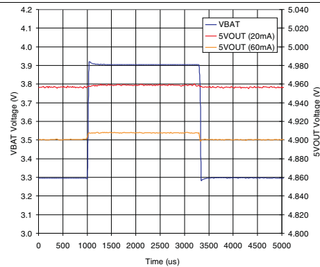
Figure 2. Line Transient Response
