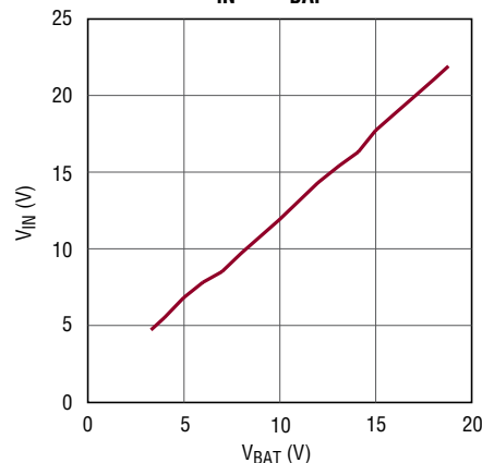
Minimum V_{IN} vs V_{BAT} 1.7A Load
