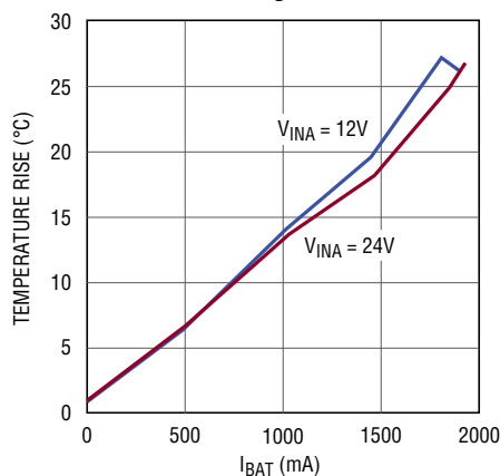
Temperature Rise vs I_{BAT} , 8.4V Float Voltage
