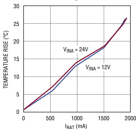
Temperature Rise vs I_{BAT} , 7.2V Float Voltage
