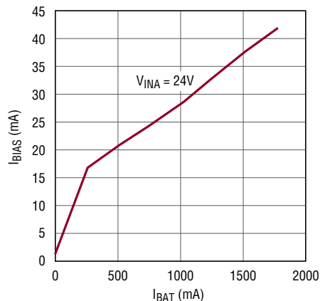
I_{\text{BIAS}} vs I_{\text{BAT}} , 14.4V Float
