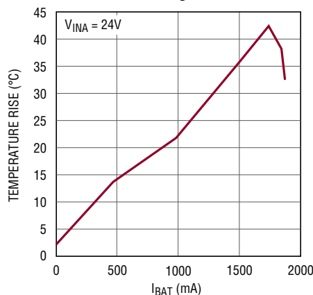
Temperature Rise vs I_{BAT} , 18.8V Float Voltage
