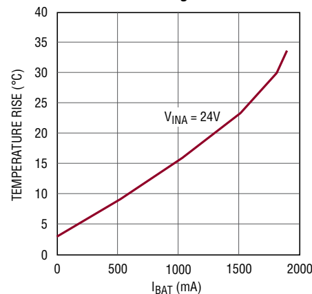
Temperature Rise vs I_{BAT} , 14.4V Float Voltage
