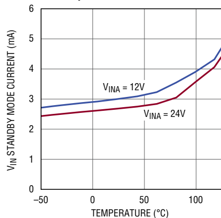
V_{IN} Standby Mode Current vs Temperature
