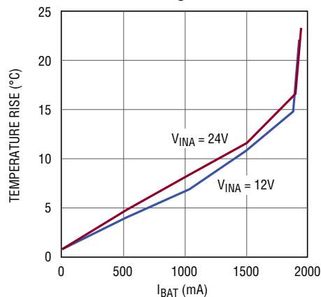
Temperature Rise vs I_{BAT} , 4.2V Float Voltage
