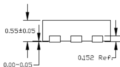
SIDE VIEW NOTE: 1, 2, 3
