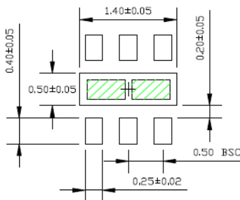
RECOMMENDED LAND PATTERN NOTE: 4
