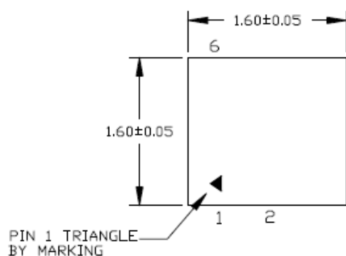
TOP VIEW NOTE: 1, 2, 3
