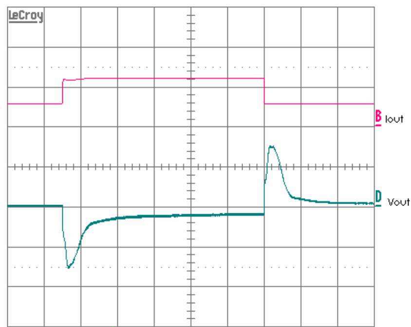
Figure 5. Transient Response Waveform at 48Vin and 5 - 6Aout – 200uS, 5A, and 200mV / div
