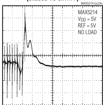
MAJOR CODE TRANSITION (0x2000 TO 0x1FFF)
