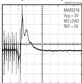
MAJOR CODE TRANSITION (0x8000 TO 0x7FFF)
