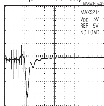
MAJOR CODE TRANSITION (0x1FFF TO 0x2000)
