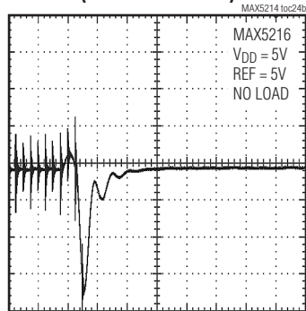
MAJOR CODE TRANSITION (0x7FFF TO 0x8000)
