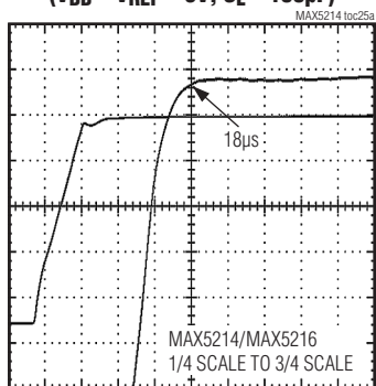
SETTLING TO ±0.5 LSB 14 BIT (V DD = V REF = 5V, C L = 100pF)
