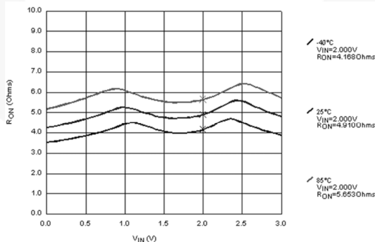
Figure 10. R_{ON} Switch On Resistance, I_{ON}=26\text{mA} , V_{CC}=3.0\text{V}
