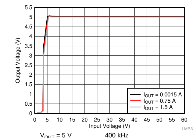
Figure 24. Line Regulation
