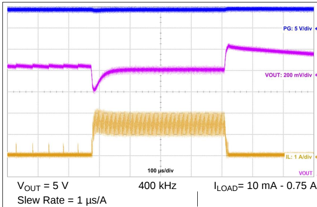
Figure 32. Load Transient
