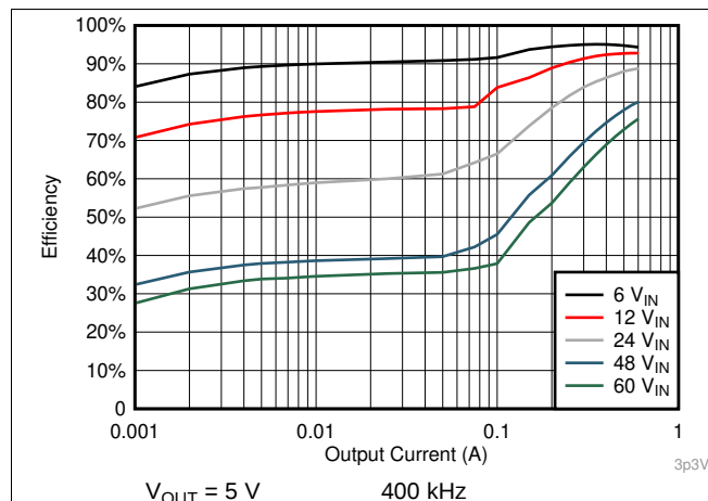
Figure 20. Efficiency
