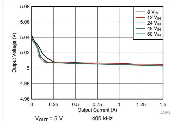
Figure 22. Load Regulation
