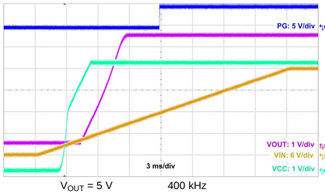
Figure 30. Start-Up Waveform
