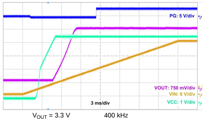
Figure 31. Start-Up Waveform
