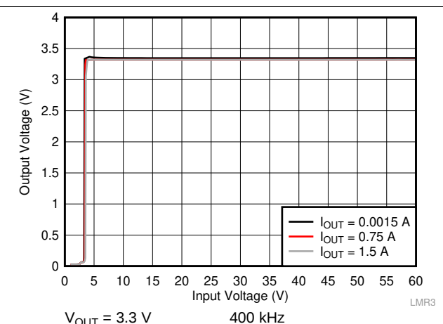
Figure 25. Line Regulation
