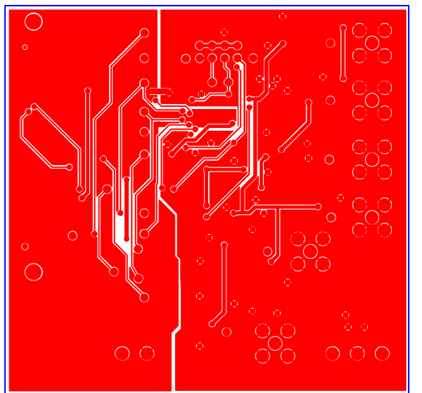
Figure 11. Solder Side
