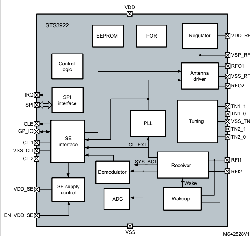
Figure 2. STS3922 block diagram
