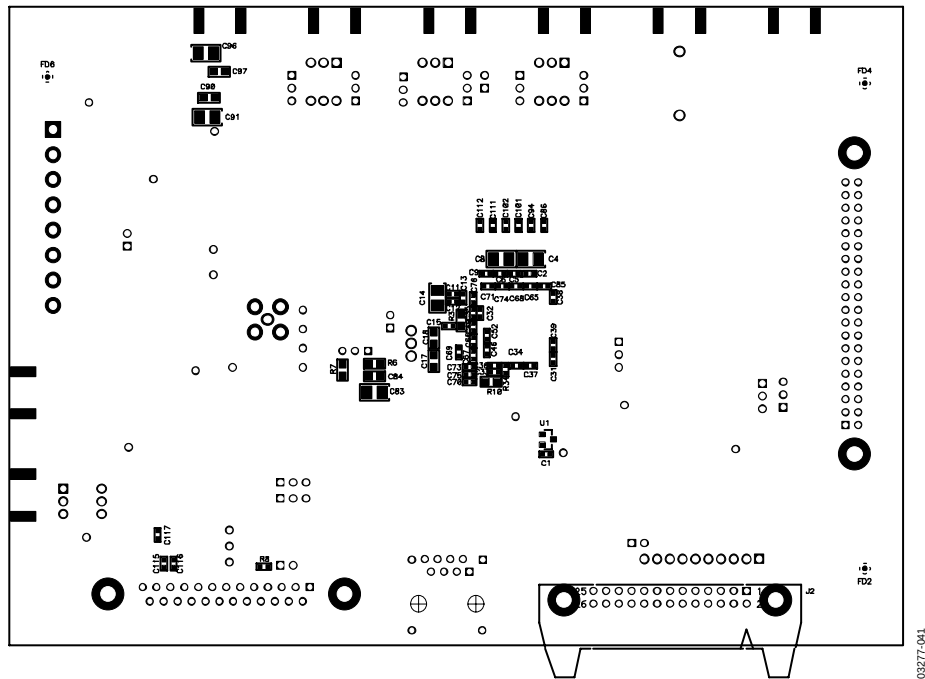
Figure 41. Evaluation PCB—Bottom Assembly
