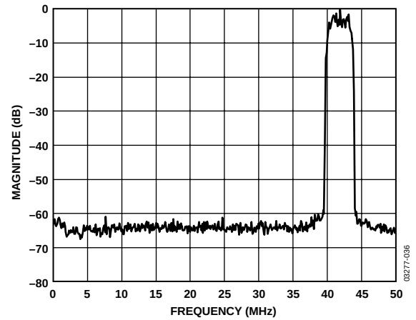
Figure 17. 16-QAM @ 42 MHz Spectral Plot, RBW = 1 kHz
