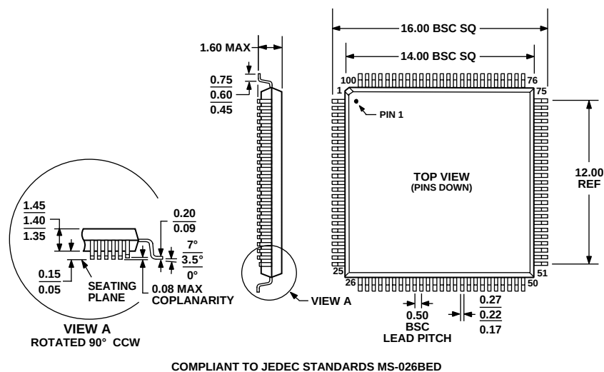
Figure 46. 100-Lead Low Profile Quad Flat Package [LQFP] (ST-100) Dimensions shown in millimeters
