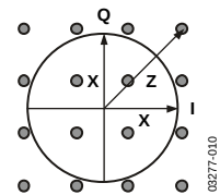
Figure 26. 16-Quadrature Modulation
