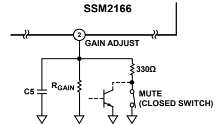
Figure 23. Details of Mute Option
