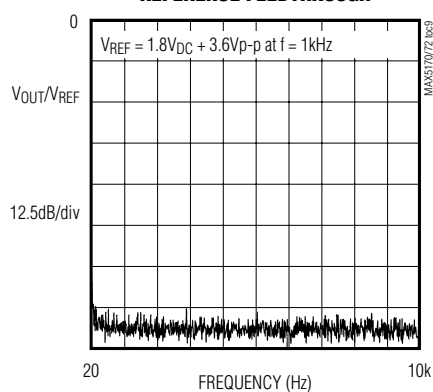
REFERENCE FEEDTHROUGH
