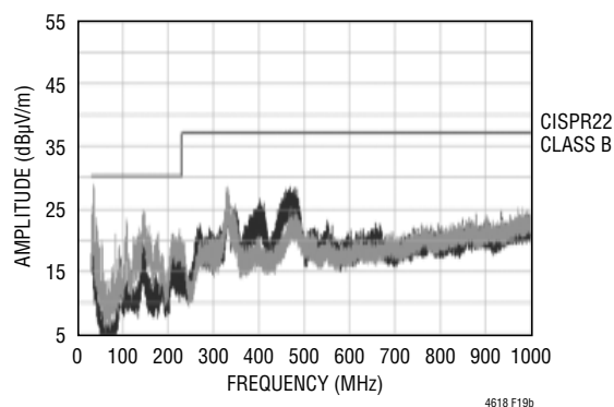
Figure 19. V_{IN} 26.5V, V_{OUT} 3.3V, I_{OUT} 5A, \pi Filter 20 \mu F to 0.22 \mu H Vishay (1616BZ) to 20 \mu F CISPR22 Radiated EMI Plots
