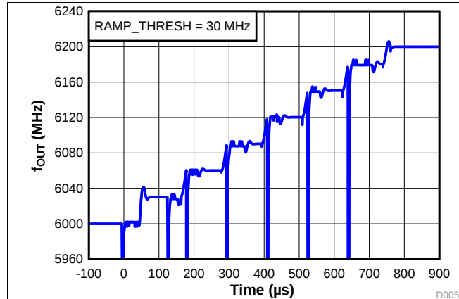
Figure 27. Automatic Ramping
