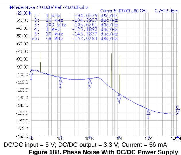
Figure 188. Phase Noise With DC/DC Power Supply
