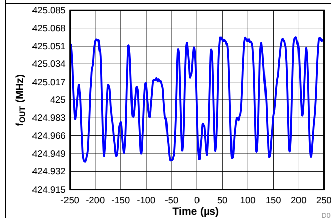
Figure 29. 4-Level GFSK Modulation
