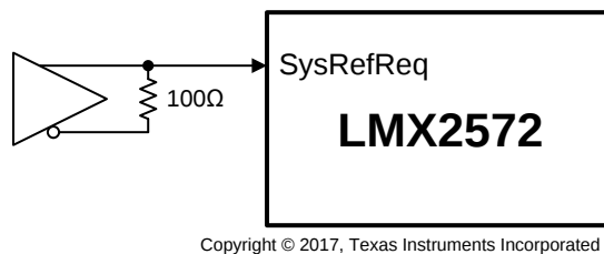
Figure 175. Driving SysRefReq Pin With Differential Signal
