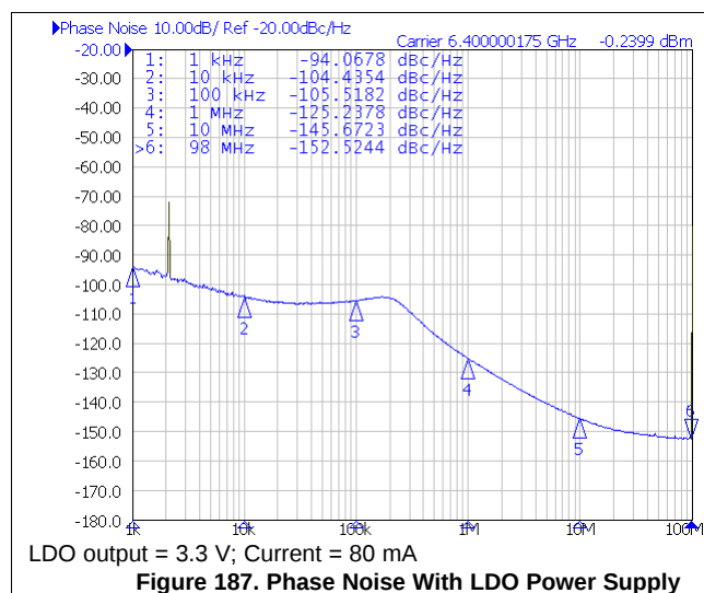
Figure 187. Phase Noise With LDO Power Supply
