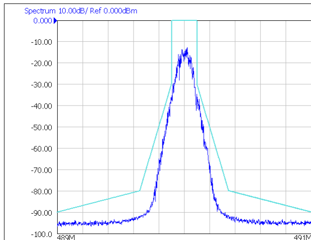
Figure 183. Gaussian 4FSK Modulated Spectrum
