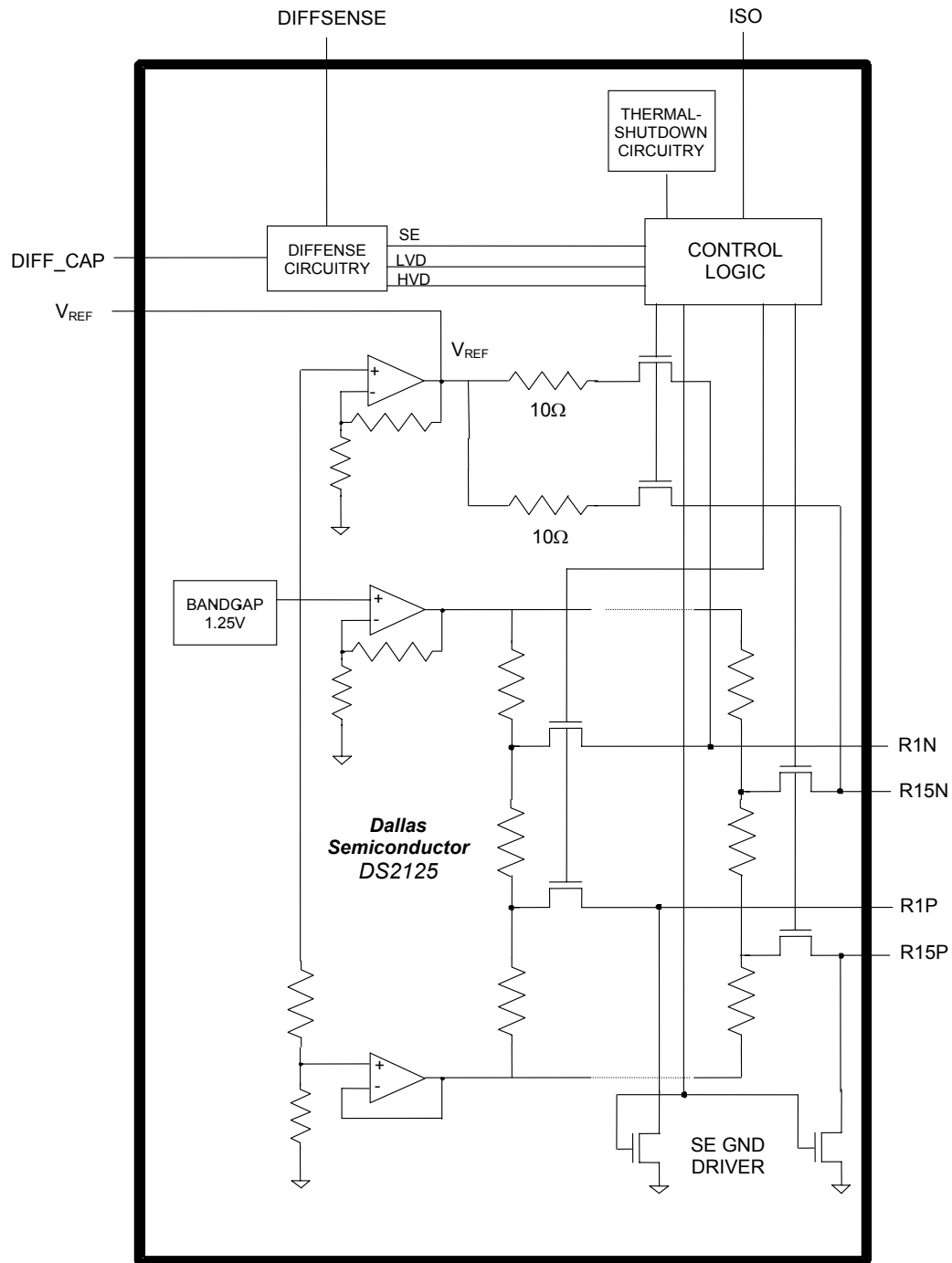
Figure 1. Block Diagram
