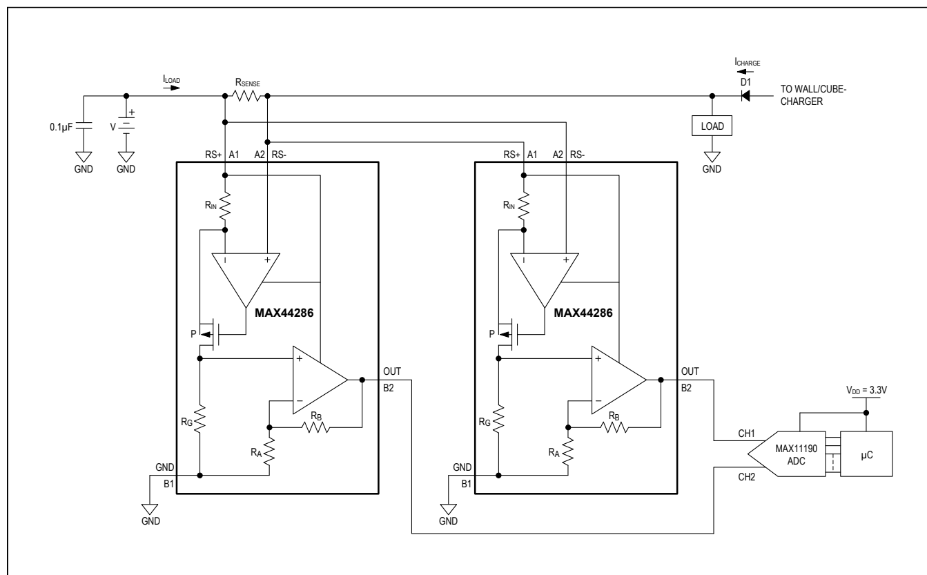
Figure 1. Bidirectional Application
