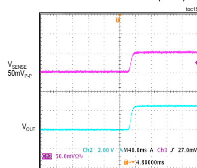
LARGE-SIGNAL RESPONSE (G = 50)
