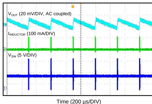
Figure 12. Eco-mode™ Operation ( V_{IN} = 12\text{ V} , V_{OUT} = 5\text{ V} , No Load)
