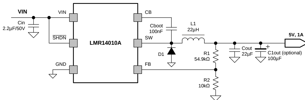
Figure 5. LMR14010A Application Circuit, 5-V Output
