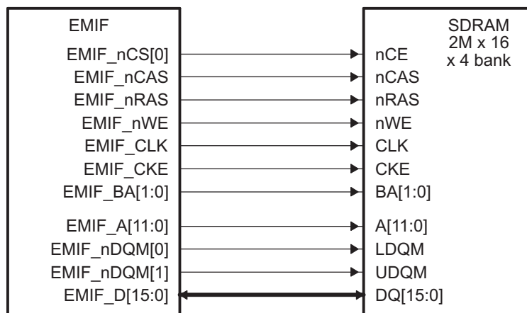
Figure 17-3. EMIF to 2\text{M} \times 16 \times 4 bank SDRAM Interface
