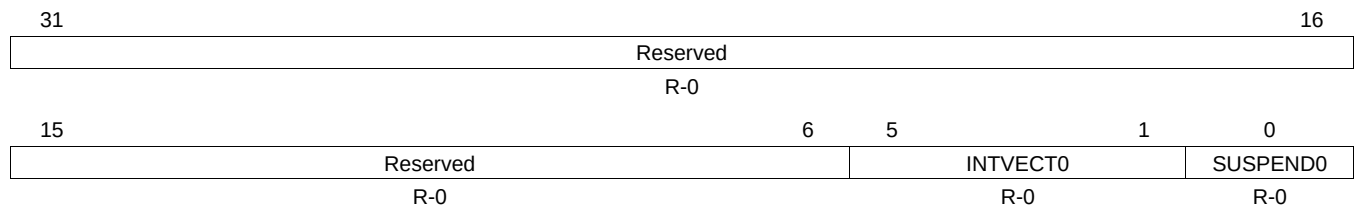
Figure 24-51. Interrupt Vector 0 (NTVECT0) [offset = 60h]
