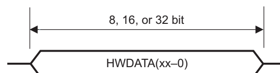
Figure 30-3. Direct Data Mode Packet Format
