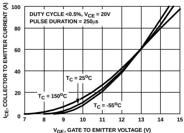
FIGURE 13. TRANSFER CHARACTERISTIC
