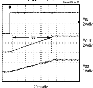
SOFT-START RESPONSE (C SS = 0.1μF)
