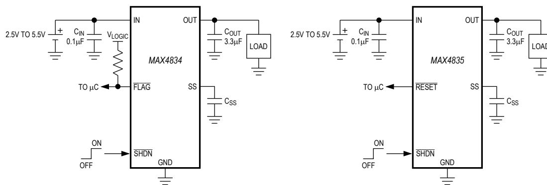
Figure 2. Typical Application Circuits
