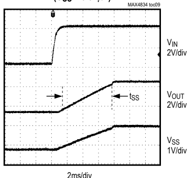
SOFT-START RESPONSE (C SS = 0.01μF)
