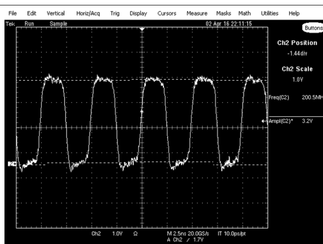
Figure 4. DS90LV012A LVCMOS Output
