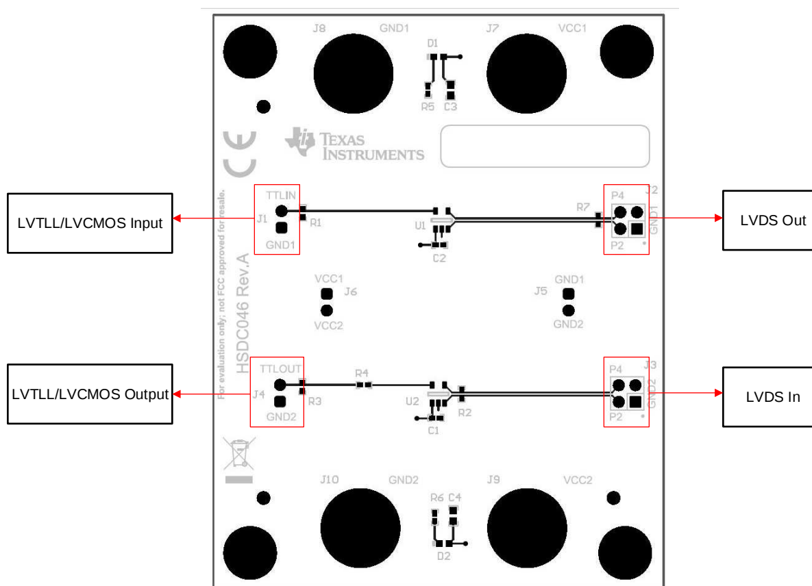
Figure 1. DS90LV011-12AEVM Input and Output Diagram
