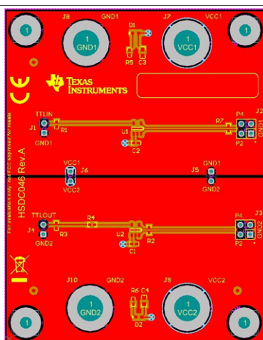
Figure 5. DS90LV011-12AEVM Top Layer
