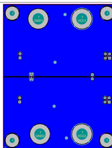
Figure 6. DS90LV011-12AEVM Bottom Layer
