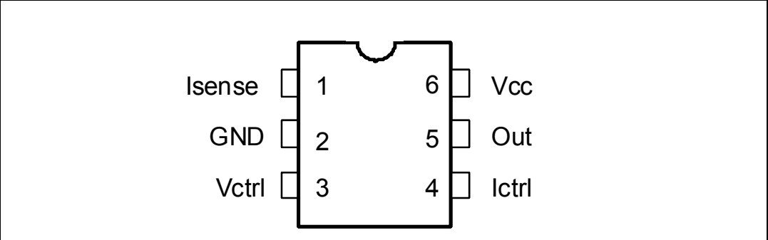
Figure 2. Pin configuration
