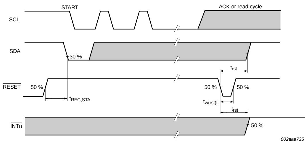
Fig 33. Definition of RESET timing
