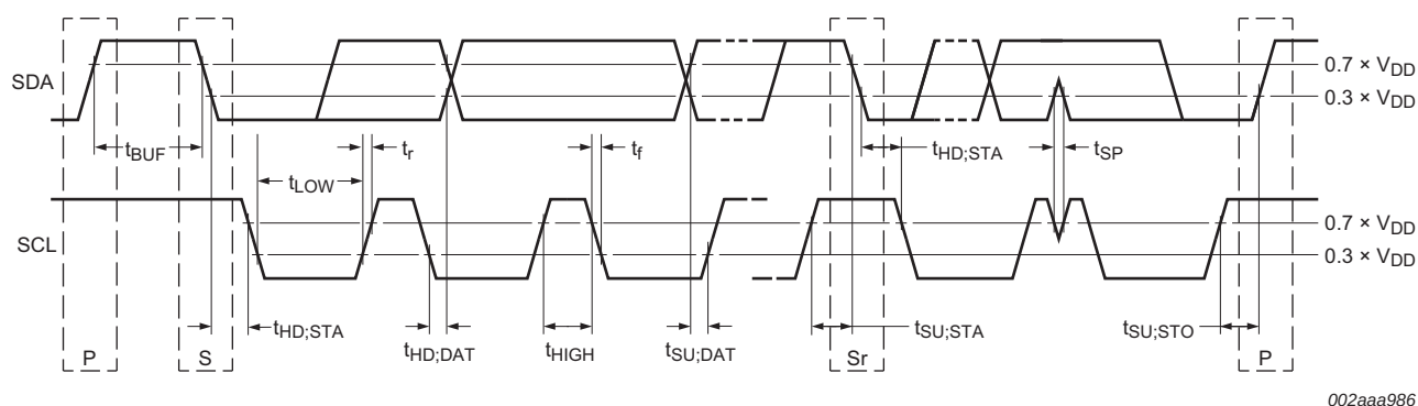
Fig 31. Definition of timing on the I 2 C-bus
