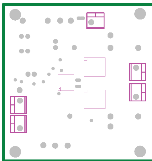
Figure 4. Layer 2
