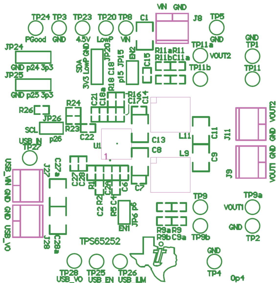
Figure 2. Top Layer
